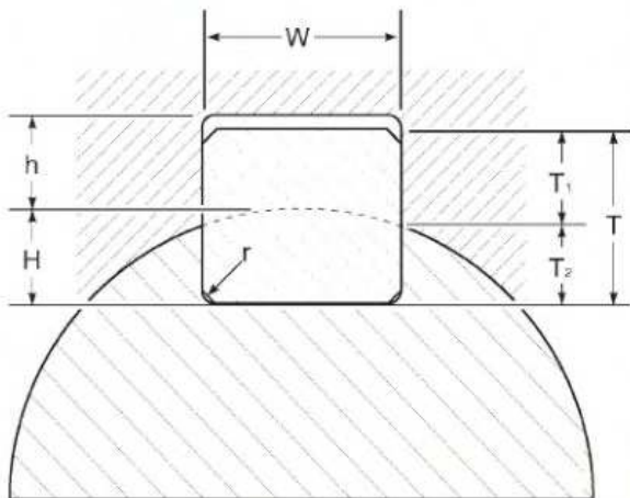
Figure 1 - Keyway and Key Size Dimension Reference
